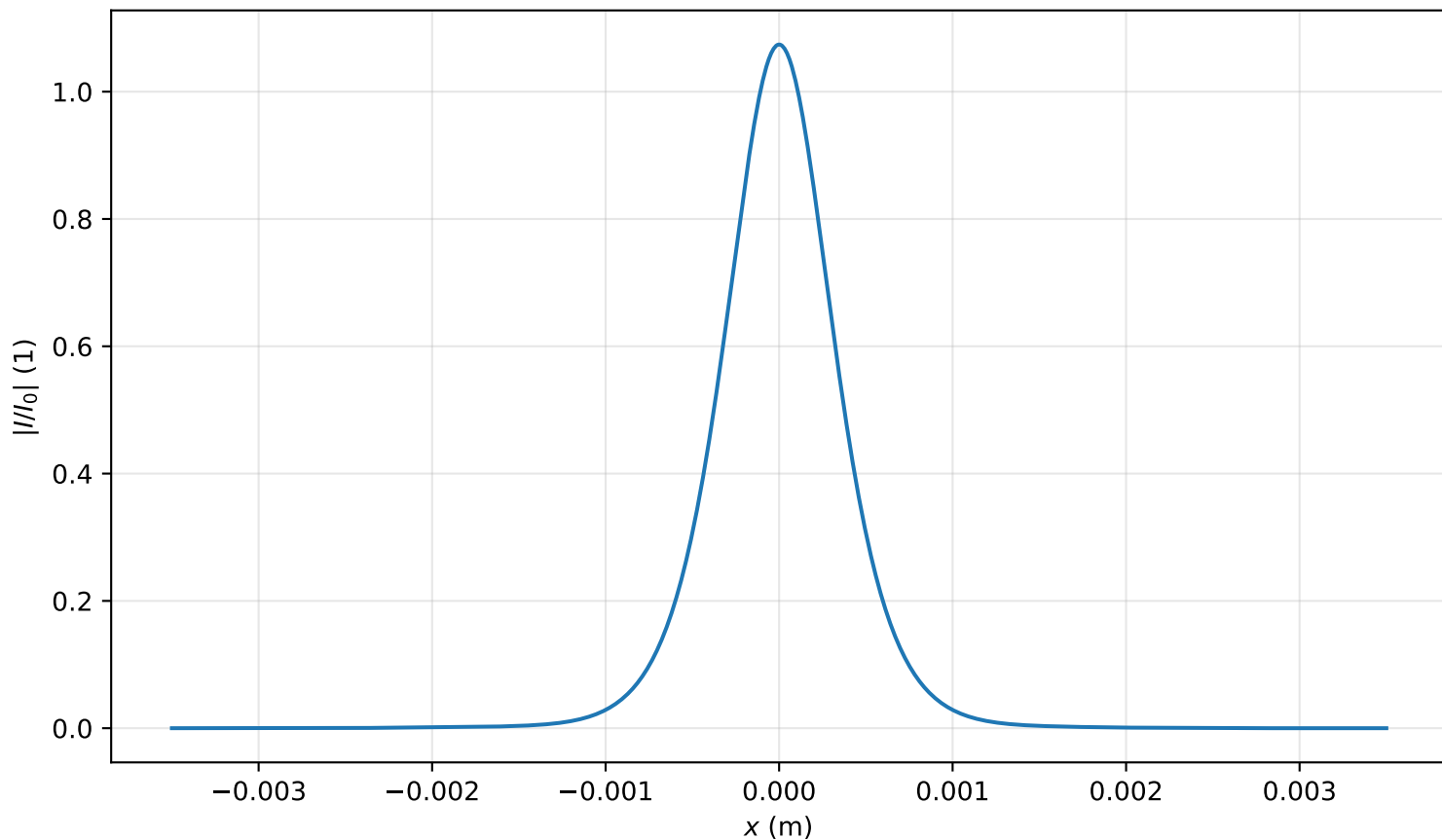
Intensity profile I(x, y = 0, z = 3.105m)/I_0 , P_{in}=0.8P_{cr} , artificial time
